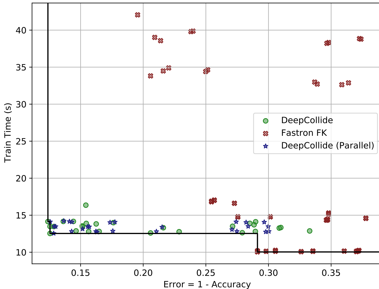
Error = (1 - Accuracy) vs. Train Time (s): 21 DoF, 30K Train, 5K Test
